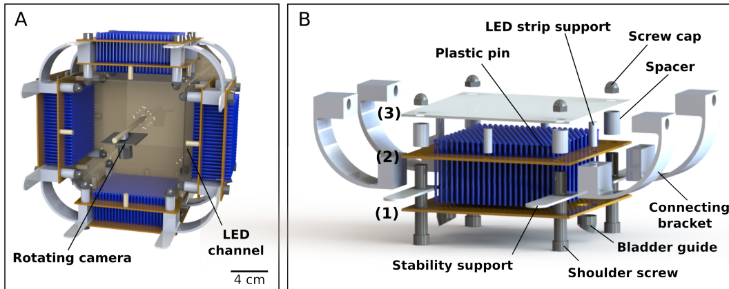
Fig. 3. Schematic of the cuboid robot. (a) Open side view, including the camera and camera mounting system (center of the robot on a dowel rod) (b) Exploded view of one face. Labels (1), (2), and (3) denote the outer, middle, and inner laser cut acrylic levels, respectively.
