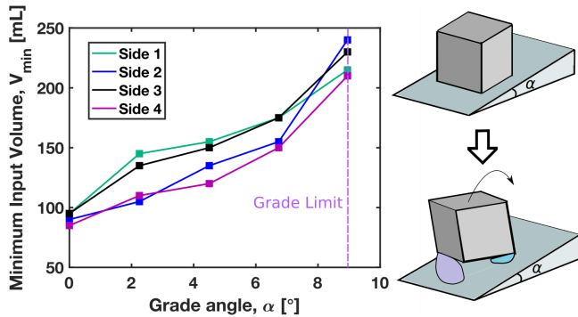
Fig. 5. The minimum volume input required to traverse sloped terrain of angle \alpha . The plotted value denotes the sum of volume required for both balloons combined, where each color denotes a different face of the cuboid. The cuboid reaches a hard limit at 9^\circ where the balloons cannot inflate enough to induce a tip.
