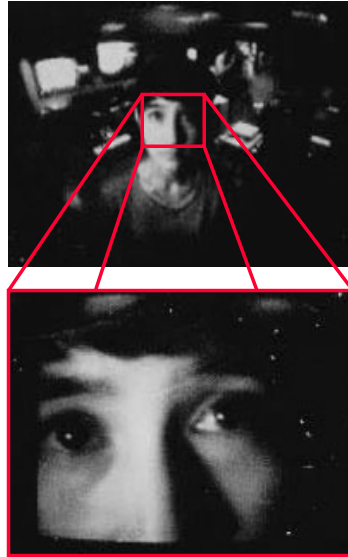
Fig. 2. Images obtained from the peripheral (top) and foveal (bottom) cameras on Cog. The peripheral image is used for detecting salient objects worthy of visual attention, while the foveal image is used to obtain high resolution detail of those objects.
